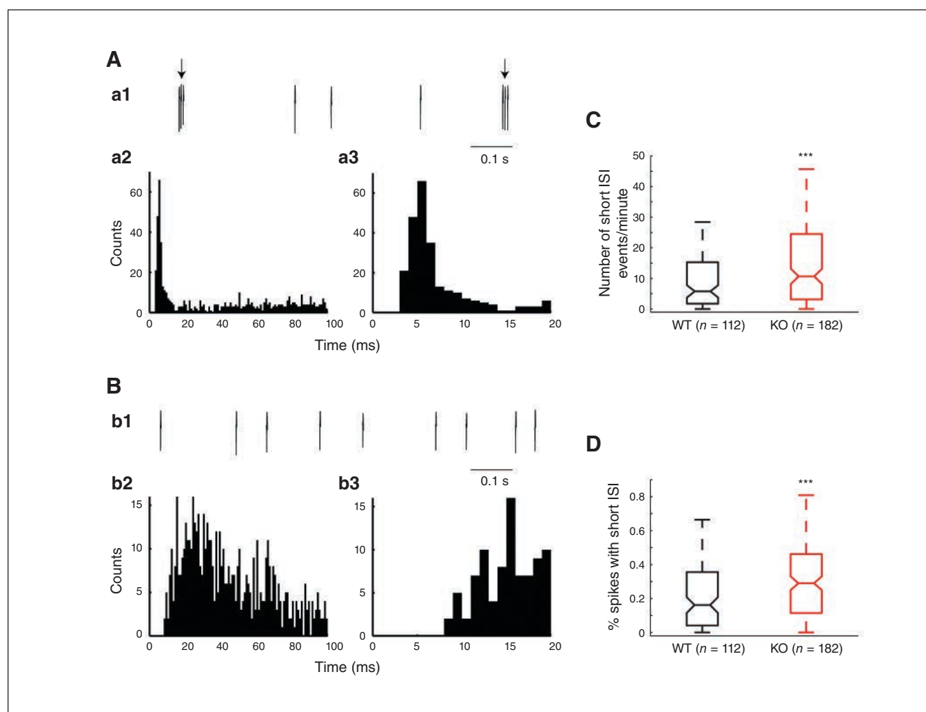
Fig. 4: The IOFC putative pyramidal neurons showed increased bursting activity in Sapap3 KO mice. (A) A representative example of bursting pyramidal neurons in Sapap3 KO mice: a1 shows the raw recording trace showing 2 bursts with short intra-burst ISI (intra-burst ISI < 10 ms, shown by arrows); a2 shows ISI distribution (bin size 1 ms); a3 shows an enlarged view of the ISI distribution from 0–20 ms to better demonstrate the short intra-burst ISI. (B) A representative example of non-bursting pyramidal neurons in Sapap3 KO mice. (C) The number of bursts per minute per neuron increased in Sapap3 KO mice; *** p = 0.001 , Wilcoxon rank sum test. (D) The percentage of spikes per neuron in the bursting mode increased in Sapap3 KO mice; *** p < 0.001 ; Wilcoxon rank sum test. The whiskers in the box plots cover 95% of the data. KO = knockout; ISI = interspike interval; IOFC = lateral orbitofrontal cortex; WT = wild type.
